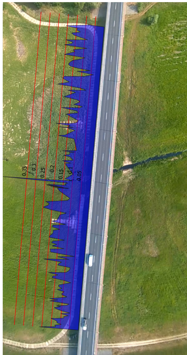
Fig. 6. Distribution of vertical averaged velocities.
