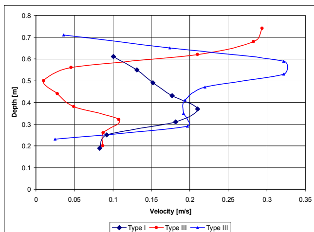
Fig. 5. Example of vertical velocity profiles.
