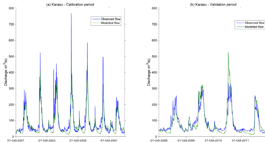
Fig. 11. SRM results in comparison to observed flows (a) Calibration period (2002–2008) (b) Validation period (2009–2012).
