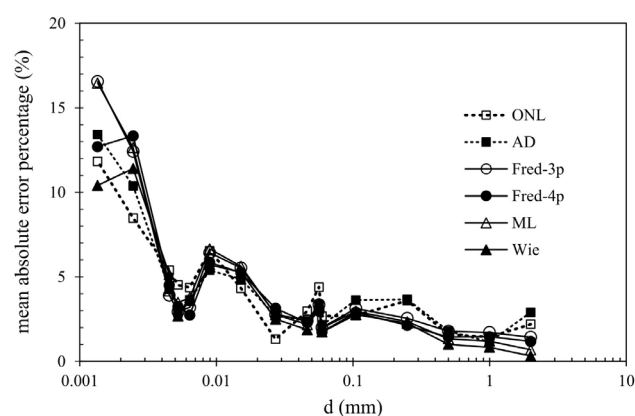
Fig. 3. Mean absolute error percentages of the six most accurate models as a function of soil particle diameter.
