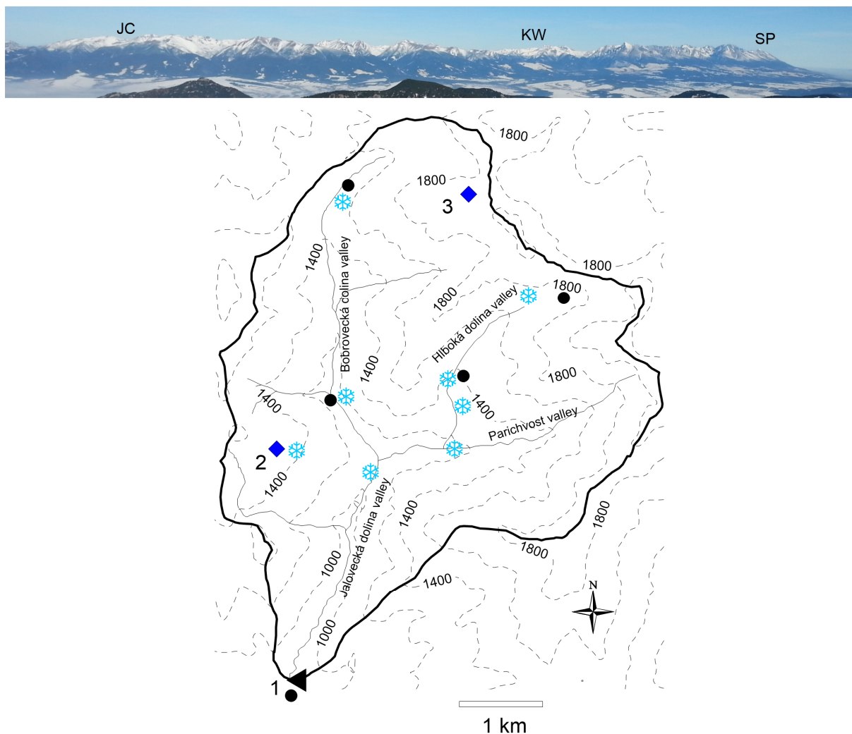
Fig. 2. Basic hydrological monitoring network in the Jalovecký Creek catchment; 1 – stream gauge (triangle) and meteorological station nearby (black circle), 2 – the main meteorological station located at catchment mean elevation, 3 – meteorological station at 1875 m a.s.l. providing the air temperature data since the hydrological year 2003; snow courses (snowflakes) and storage gauges (1989–2008; black circle), water divide (thick black line) and contour lines; the photo on the top gives an idea on the approximate distance of the Jalovecký Creek Catchment (JC) from meteorological stations at Kasprowy Wierch (KW, 20 km) and Skalnaté Pleso (SP, 38 km).
