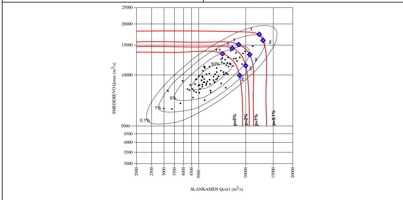
Fig. 5.1/3. Coincidence of maximum annual discharges of the Danube at HS Smederevo and corresponding discharges of the Danube at HS Slankamen
