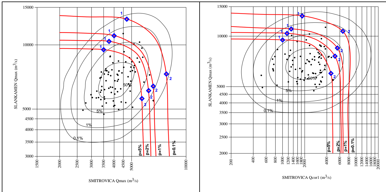
Fig. 5.2/2. Coincidence of maximum annual discharges of the Danube at HS Slankamen and corresponding discharges of the Sava at HS Sremska Mitrovica
