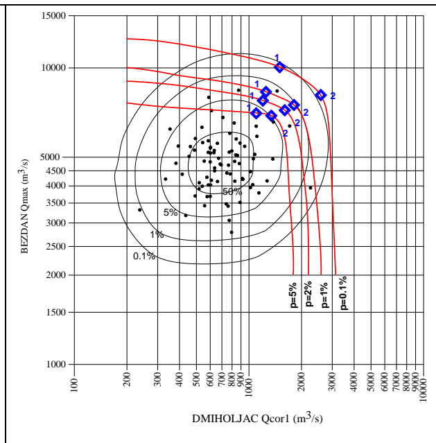
Fig. 3.2/2. Coincidence of maximum annual discharges of the Danube at HS Bezdán and corresponding discharges of the Drava at HS Donji Miholjac
