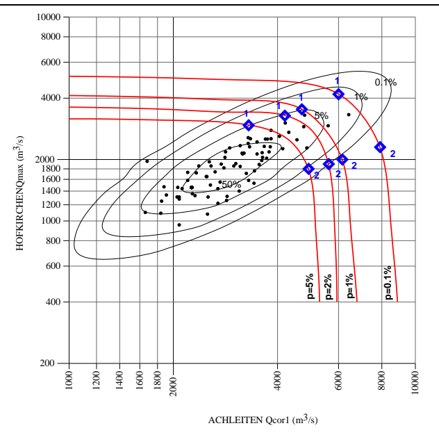
Fig. 1.1/2. Coincidence of maximum annual discharge of the Danube at HS Hofkirchen and corresponding discharge of the Danube at HS Achleiten
