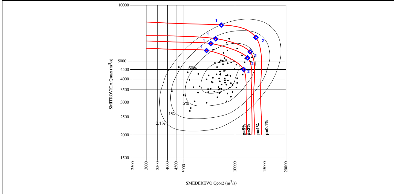
Fig. 5.3/3. Coincidence of maximum annual discharges of the Sava at HS Sremska Mitrovica and corresponding discharges of the Danube at HS Smederevo
