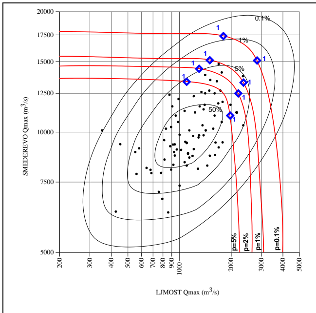
Fig. 6.2/1. Coincidence of maximum annual discharges of the Danube at HS Smederevo and maximum annual discharges of the Velika Morava at HS Ljubičevski Most
