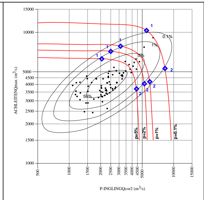
Fig. 1.3/2. Coincidence of maximum annual discharges of the Danube at HS Achleiten and corresponding discharges of the Inn at HS P-Ingling
