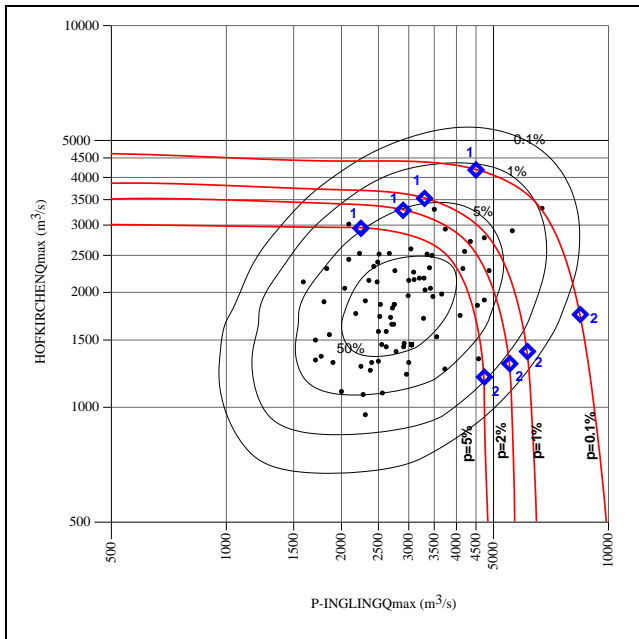
Fig. 1.2/1. Coincidence of maximum annual discharges of the Danube at HS Hofkirchen and maximum annual discharges of the Inn at HS P-Ingling
