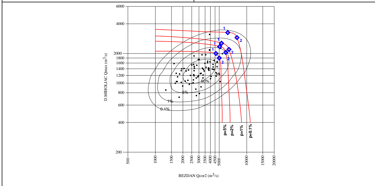
Fig. 3.2/3. Coincidence of maximum annual discharges of the Drava at HS Donji Miholjac and corresponding discharges of the Danube at HS Bezdán
