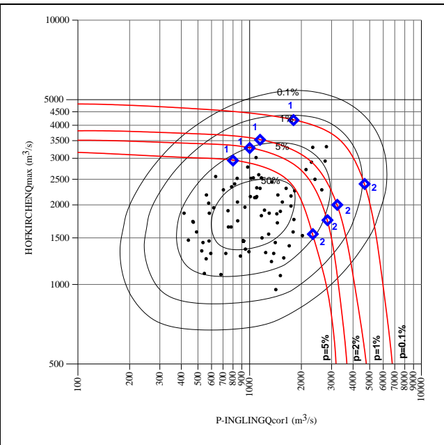
Fig. 1.2/2. Coincidence of maximum annual discharges of the Danube at HS Hofkirchen and corresponding discharges of the Inn at HS P-Ingling
