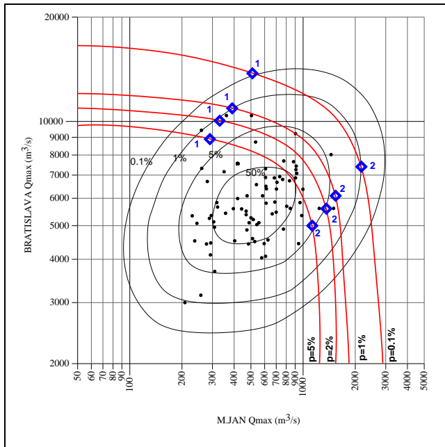
Fig. 2.3/1. Coincidence of maximum annual discharges of the Danube at HS Bratislava and maximum annual discharges of the Morava at HS Moravsky Jan
