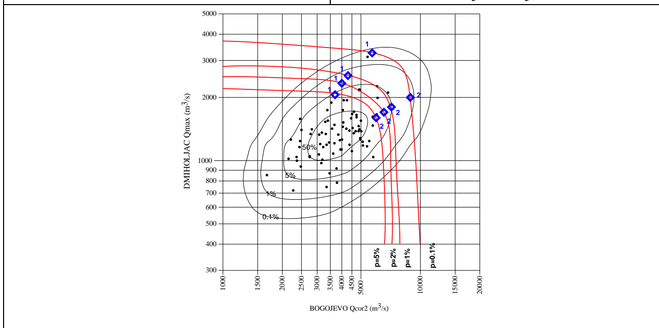
Fig. 3.3/2. Coincidence of maximum annual discharges of the Danube at HS Bogojevo and corresponding discharges of the Drava at HS Donji Miholjac
