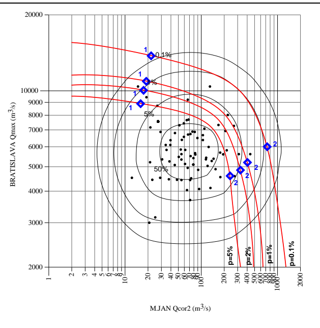
Fig. 2.3/2. Coincidence of maximum annual discharges of the Danube at HS Bratislava and corresponding discharges of the Morava at HS Moravsky Jan
