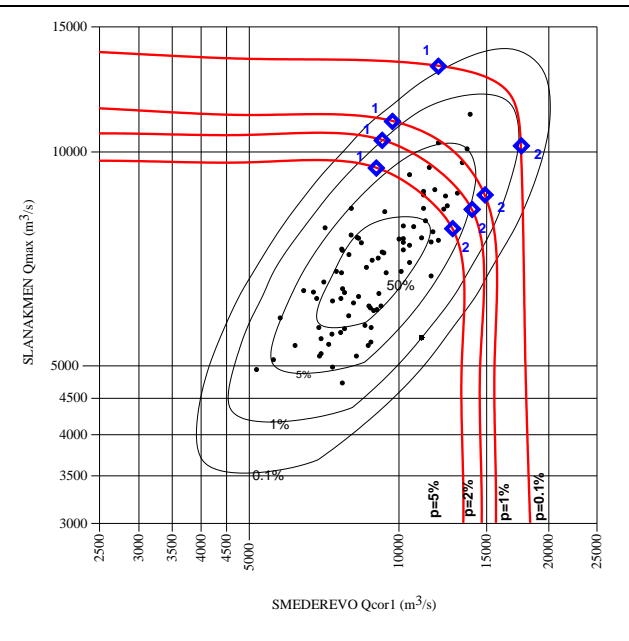
Fig. 5.1/2. Coincidence of maximum annual discharge of the Danube at HS Slankamen and corresponding discharge of the Danube at HS Smederevo
