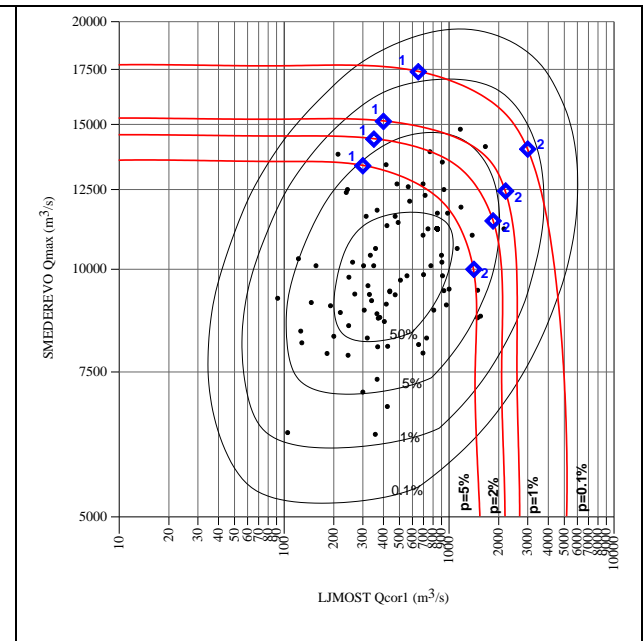
Fig. 6.2/2. Coincidence of maximum annual discharges of the Danube at HS Smederevo and corresponding discharges of the Velika Morava at HS Ljubičevski Most
