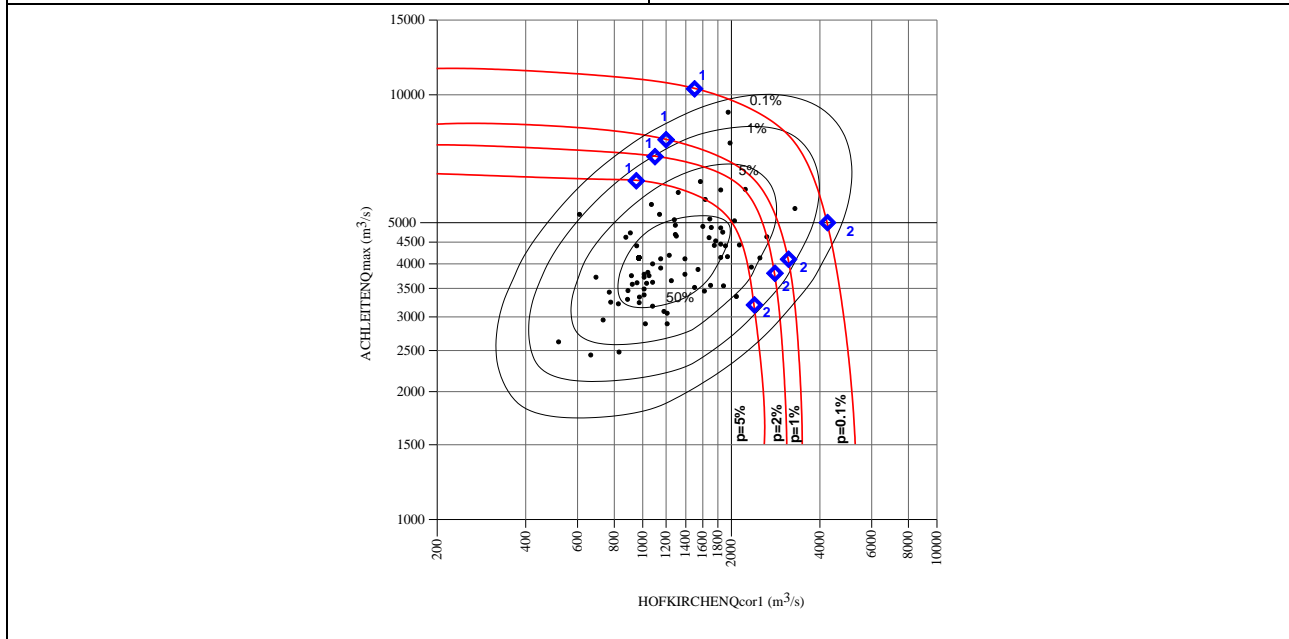
Fig. 1.1/3. Coincidence of maximum annual discharges of the Danube at HS Achleiten and corresponding discharges of the Danube at HS Hofkirchen
