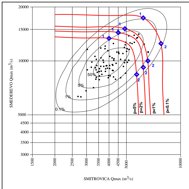
Fig. 5.3/1. Coincidence of maximum annual discharges of the Danube at HS Smederevo and maximum annual discharges of the Sava at HS Sremska Mitrovica
