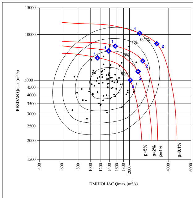
Fig. 3.2/1. Coincidence of maximum annual discharges of the Danube at HS Bezdán and maximum annual discharges of the Drava at HS Donji Miholjac
