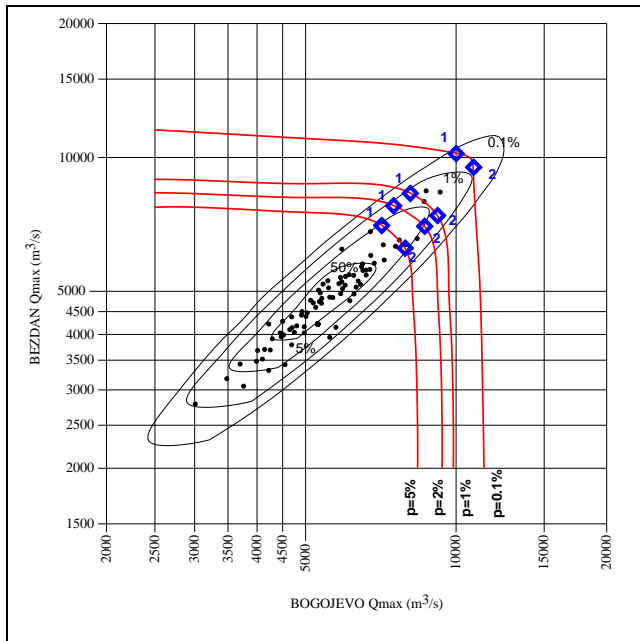
Fig. 3.1/1. Coincidence of maximum annual discharges of the Danube at HS Bezdán and HS Bogojevo
