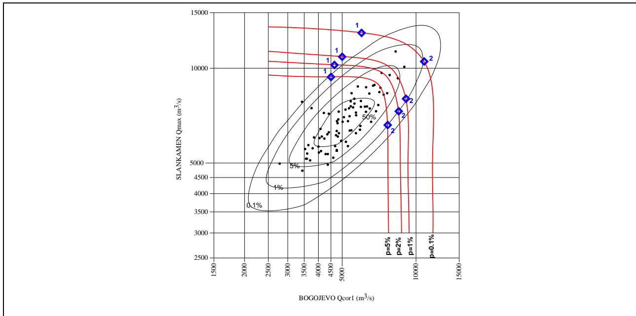
Fig. 4.1/3. Coincidence of maximum annual discharges of the Danube at HS Slankamen and corresponding discharges of the Danube at HS Bogojevo
