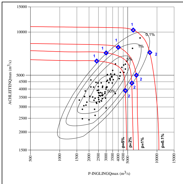
Fig. 1.3/1. Coincidence of maximum annual discharges of the Danube at HS Achleiten and maximum annual discharges of the Inn at HS P-Ingling
