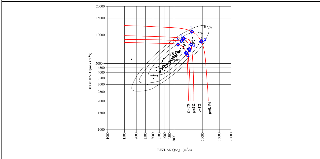
Fig. 3.1/3. Coincidence of maximum annual discharges of the Danube at HS Bogojevo and corresponding discharges of the Danube at HS Bezdán
