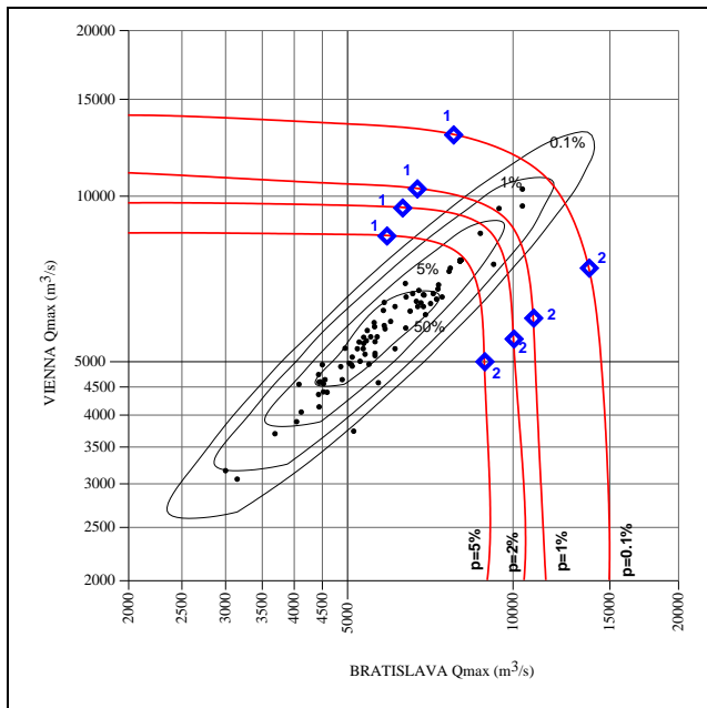
Fig. 2.1/1. Coincidence of maximum annual discharges of the Danube at HS Vienna and HS Bratislava
