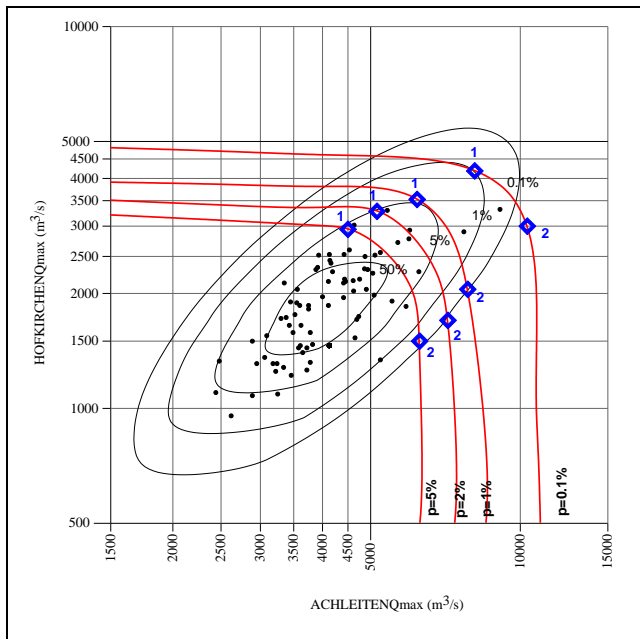
Fig. 1.1/1. Coincidence of maximum annual discharges of the Danube at HS Hofkirchen and HS Achleiten
