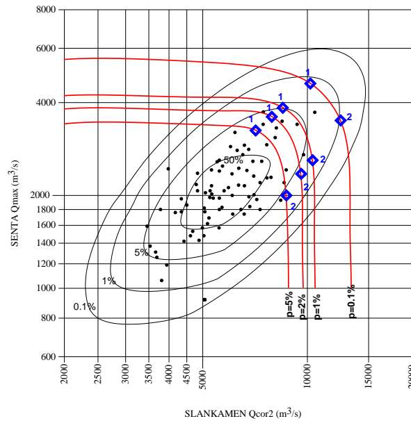
Fig. 4.3/3. Coincidence of maximum annual discharges of the Tisa at HS Senta and corresponding discharges of the Danube at HS Slankamen
