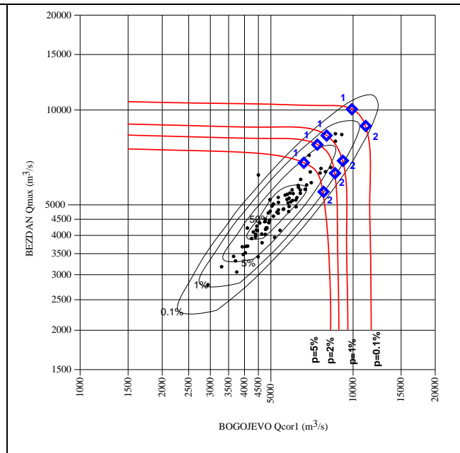
Fig. 3.1/2. Coincidence of maximum annual discharge of the Danube at HS Bezdán and corresponding discharge of the Danube at HS Bogojevo
