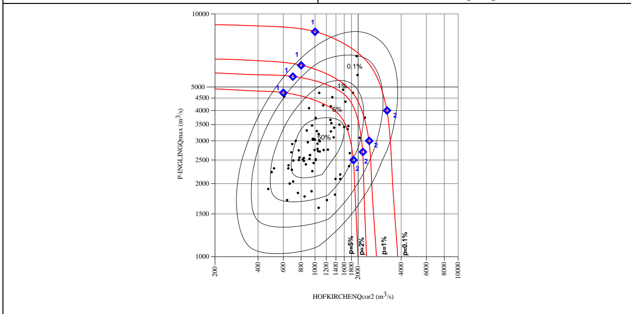
Fig. 1.2/1. Coincidence of maximum annual discharges of the Danube at HS Hofkirchen and maximum annual discharges of the Inn at HS P-Ingling
