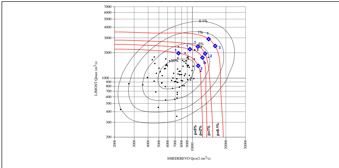
Fig. 6.2/3. Coincidence of maximum annual discharges of the Velika Morava at HS Ljubičevski Most and corresponding discharges of the Danube at HS Smederevo
