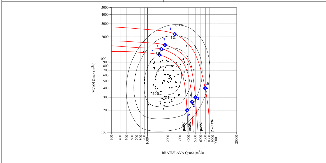
Fig. 2.3/3. Coincidence of maximum annual discharges of the Morava at HS Moravsky Jan and corresponding discharges of the Danube at HS Bratislava
