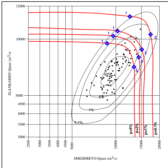
Fig. 5.1/1. Coincidence of maximum annual discharges of the Danube at HS Slankamen and HS Smederevo
