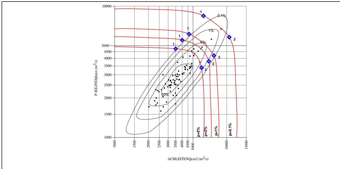
Fig. 1.3/3. Coincidence of maximum annual discharges of the Inn at HS P-Ingling and corresponding discharges of the Danube at HS Achleiten
