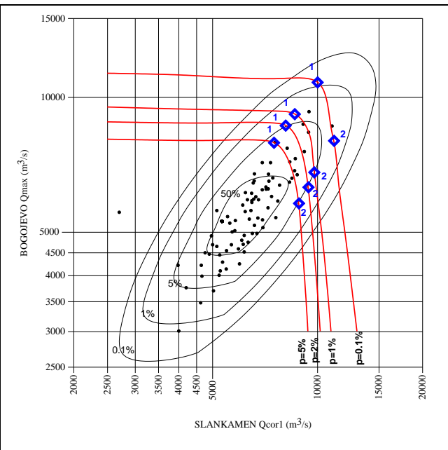
Fig. 4.1/2. Coincidence of maximum annual discharge of the Danube at HS Bogojvo and corresponding discharge of the Danube at HS Slankamen
