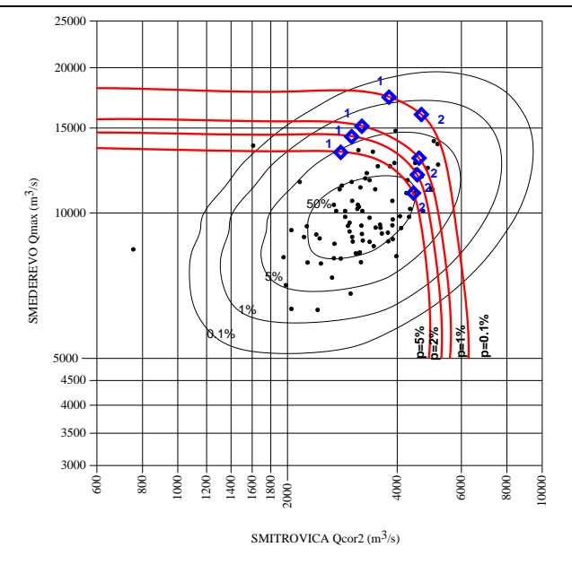
Fig. 5.3/2. Coincidence of maximum annual discharges of the Danube at HS Smederevo and corresponding discharges of the Sava at HS Sremska Mitrovica
