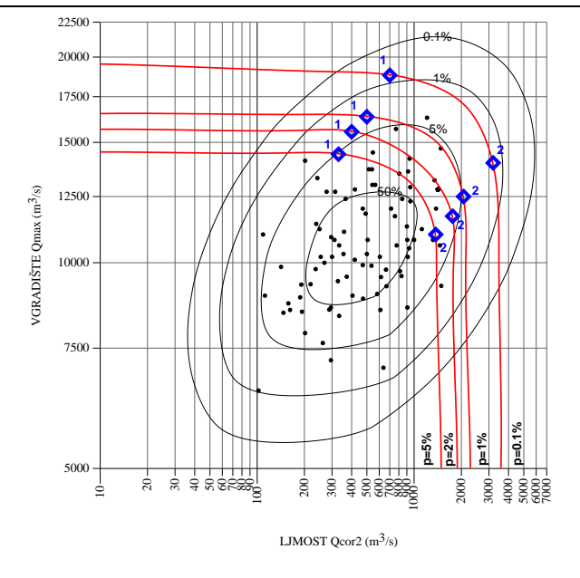
Fig. 6.3/2. Coincidence of maximum annual discharges of the Danube at HS Veliko Gradište
