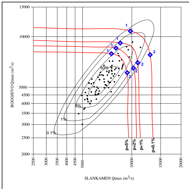
Fig. 4.1/1. Coincidence of maximum annual discharges of the Danube at HS Bogojvo and HS Slankamen
