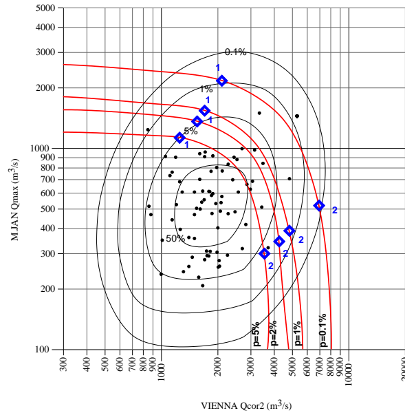
Fig. 2.2/3. Coincidence of maximum annual discharges of the Morava at HS Moravsky Jan and corresponding discharges of the Danube at HS Vienna
